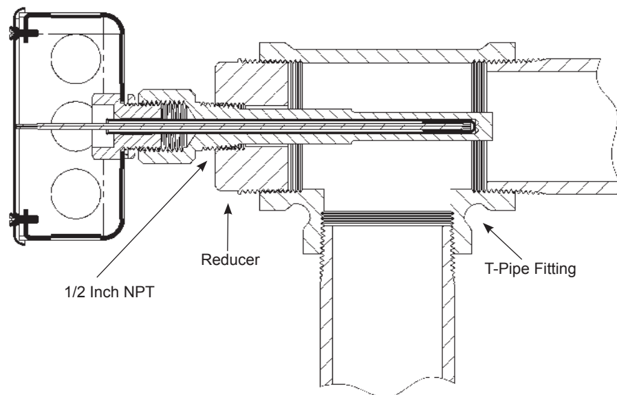
Fig 5: Typical Corner Mount
