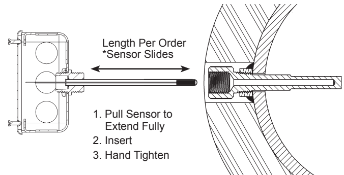
Fig 6: Immersion Sensor Before Insertion
