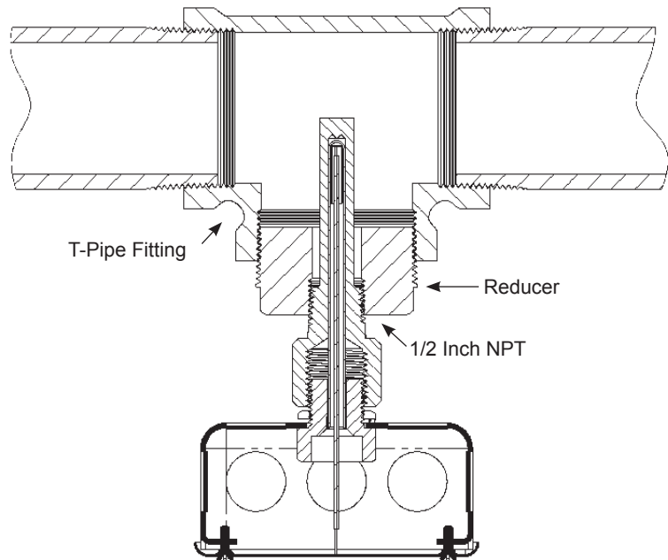
Fig 4: Typical T-Mount
