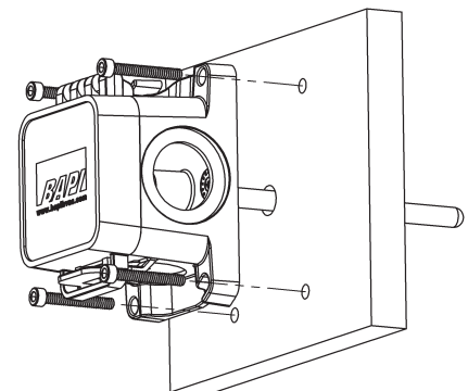
Fig. 3: BAPI-Box Crossover Mounting to the Duct
